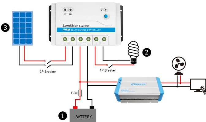
Figure 2 Connection diagram
