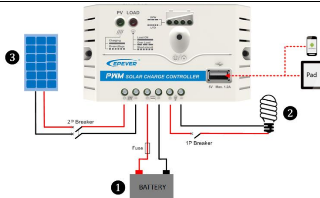
Figure 2 Connection diagram
